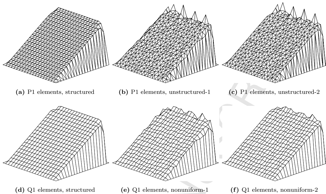
Figure 3: FIC-FEM solution to Example 2. \mathbf{v} = [1, 0]^T , k_1 = 10^{-8} , k_2 = 10^{-8} , s = 0 , Q = 1 and viewed at (-45^\circ, 20^\circ) .
